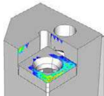
Poor clamping strength due to single directional force
