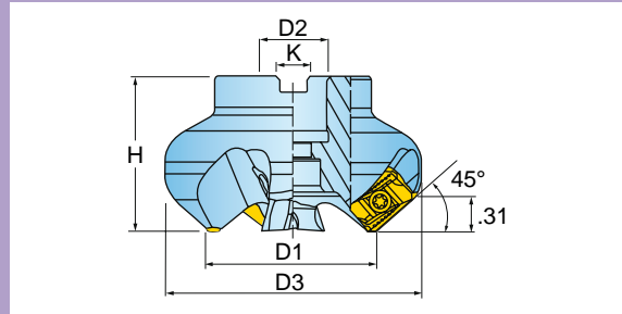
Chamfer
