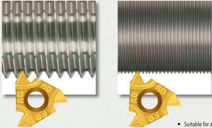
Partial Profile
