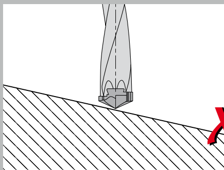
Angular or Irregular Surfaces (Maximum 6° angle)
