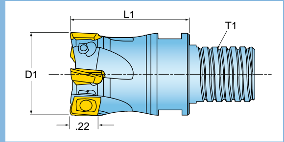
Shoulder
