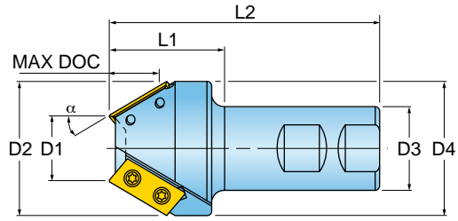
Chamfer
