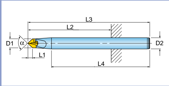
Spot Drilling
