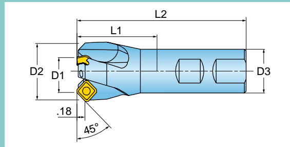
Facing
