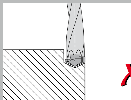
Interrupted or Partial Holes
