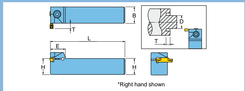
Face turning
