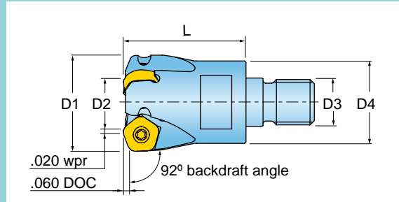
Ramping
