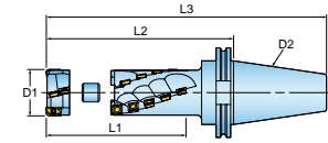
Drawing B- Face Mounted Style
