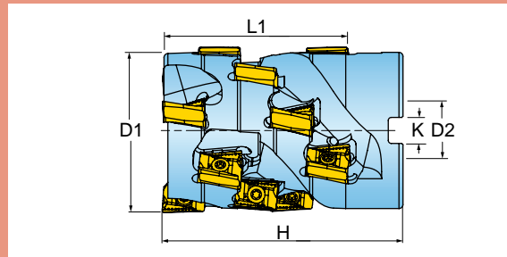
Slabbing
