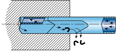
Gun drilling operation in blind hole when chips and coolant are evacuated back through the flute.
