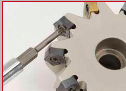
Long bit for traditional mounted inserts.
